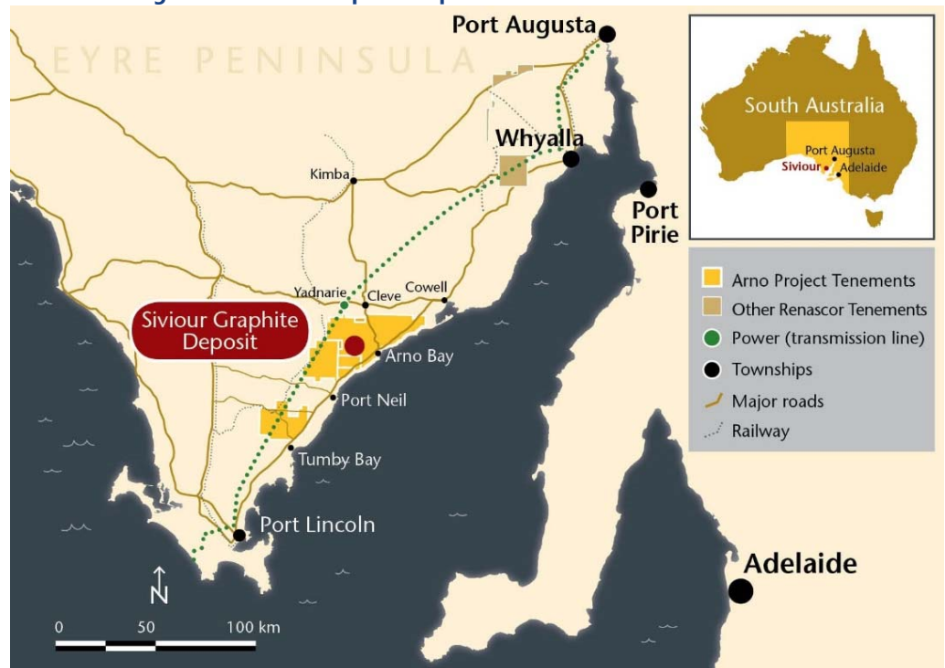
Figure 1. Siviour Graphite Deposit
