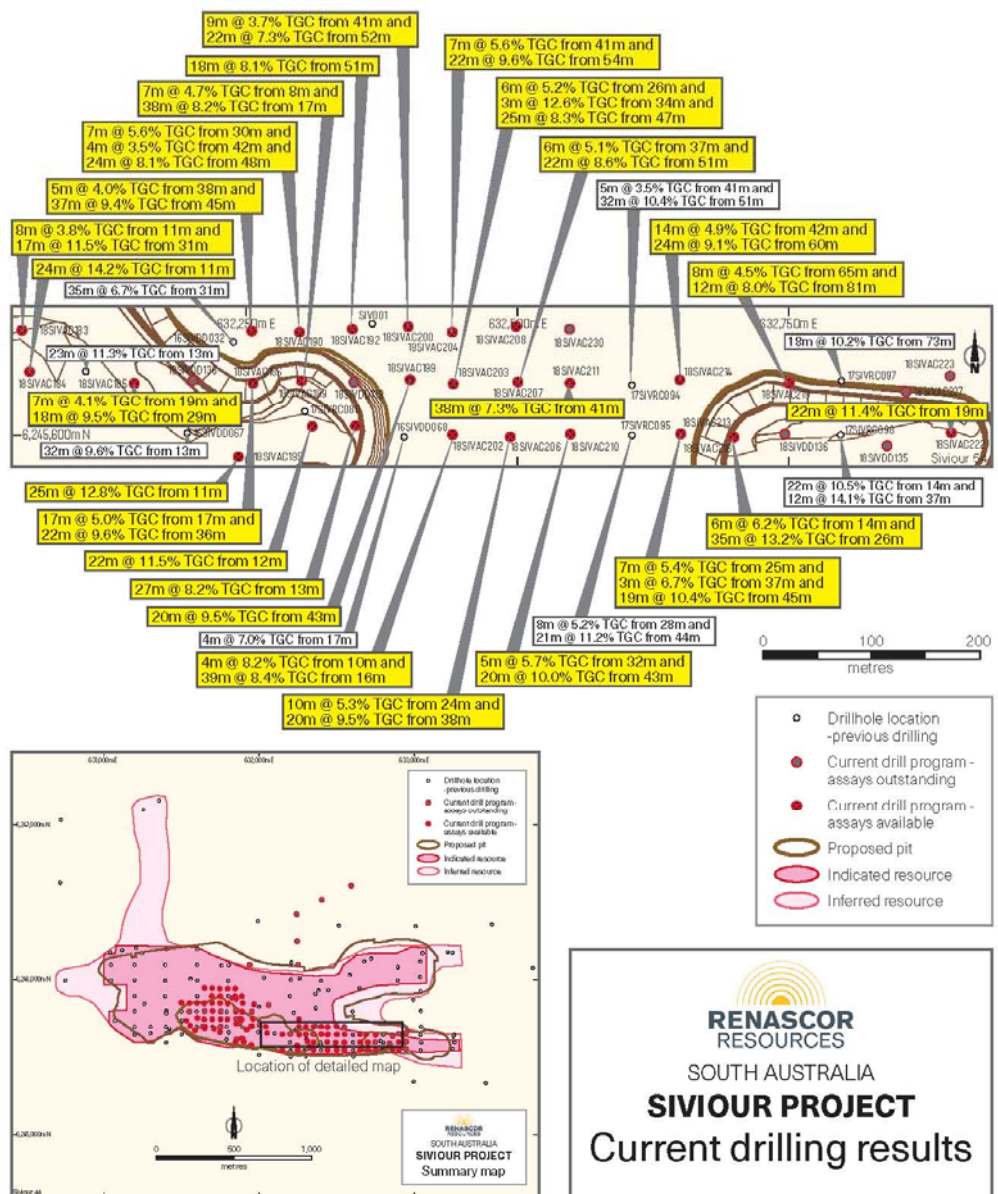
Figure 2. Siviour Graphite Project, showing significant drill intercepts from newly available assays (in yellow) in relation to PFS initial pit designs
