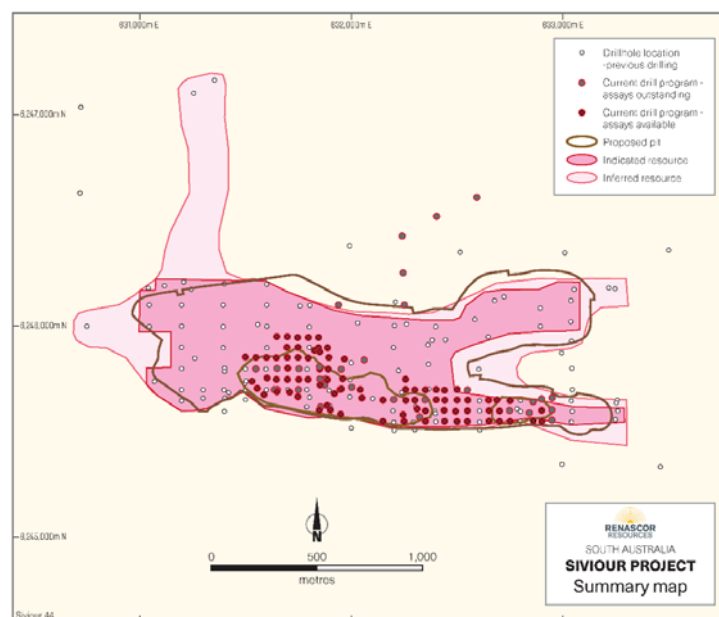
Figure 1. Siviour Graphite Project, showing recently drilled holes in relation to previously drilled holes, Indicated and Inferred Resource outlines and proposed pit design
