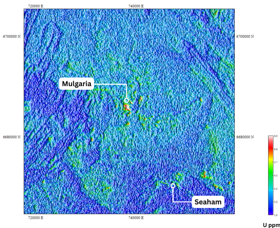
Figure 9. Comparison of the Mulgaria anomalous radiometric response (approximately 2 km by 1 km in size, total image area approximately 1,600km 2 ) to nearby Seaham uranium prospect, with Mulgaria presenting as a stand-out uranium channel radiometrics feature, depicted as a white peak where GCAS values are above an estimated 8ppm uranium (radiometrics)
