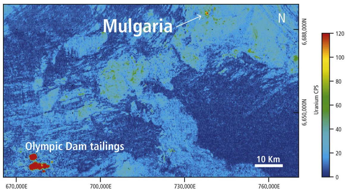
Figure 10. Regional-scale GCAS image approximately 100km by 75km (7,500km 2 ) comparing the Mulgaria radiometric response to the Olympic Dam complex, depicted as red peaks where GCAS values are above 110 counts per second (CPS) uranium
