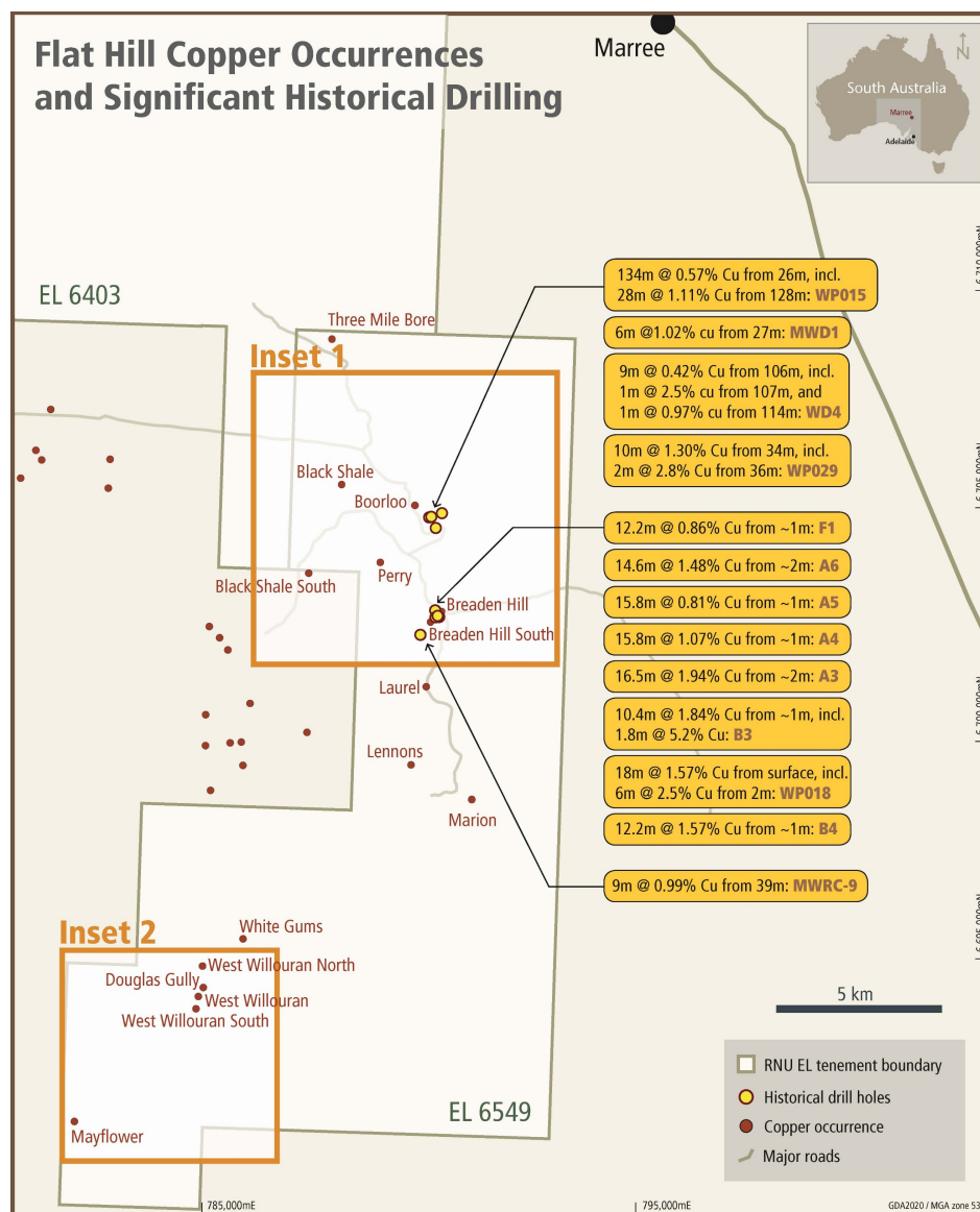
Figure 6. Flat Hill prospect area, showing historical mineral occurrences and significant drill intersections 16 . Newly identified VTEM targets are shown in Figures 7 and 8, labelled above as Inset 1 and Inset 2 respectively
