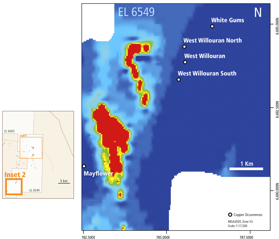
Figure 8. VTEM image showing defined (late-time SFz45) exploration targets within southern portion of Flat Hill 19 . See Inset 2 for location
