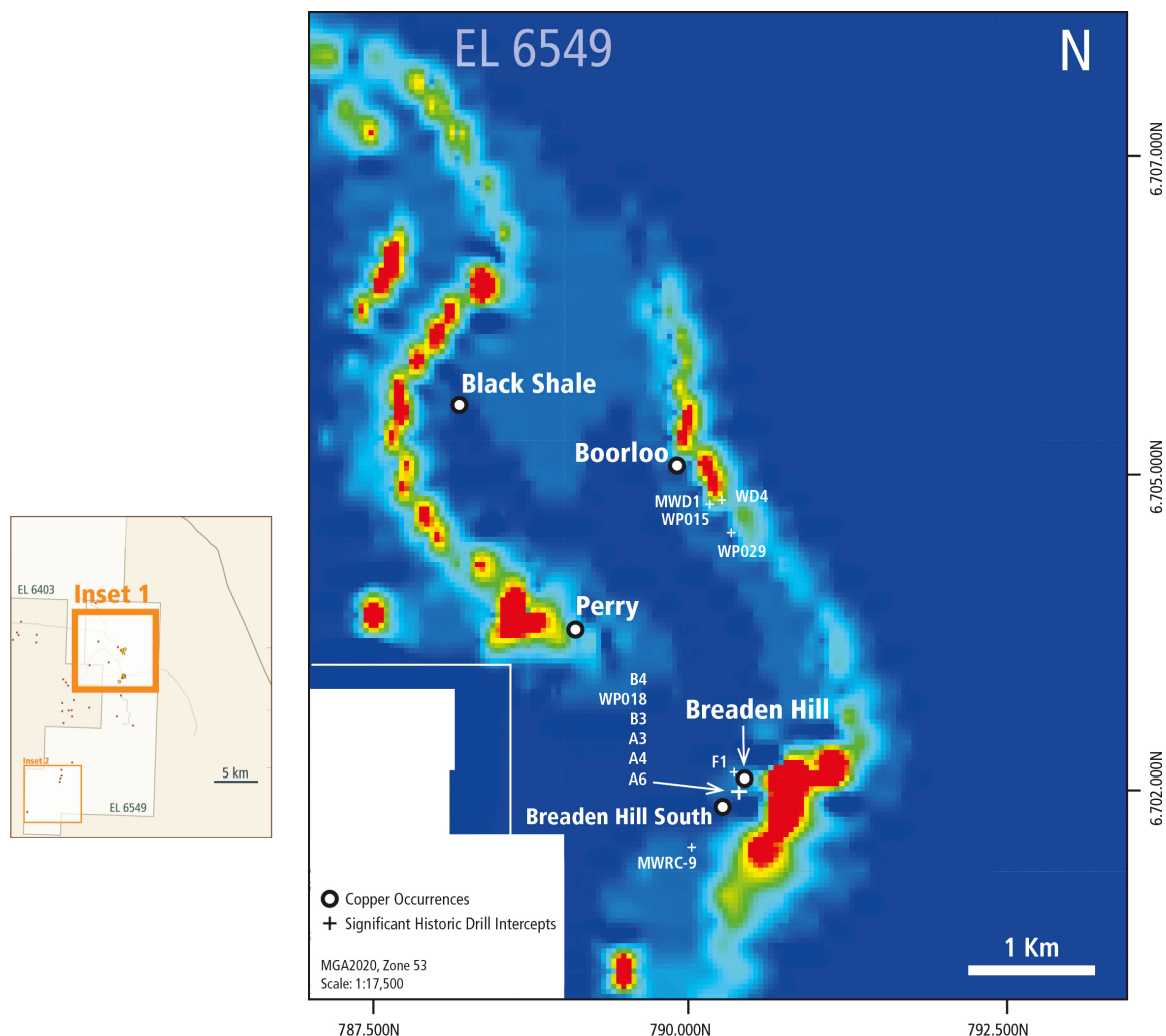
Figure 7. VTEM image showing defined (late-time SFz45) exploration targets identified within northern portion of Flat Hill 18 . See Inset 1 for location
